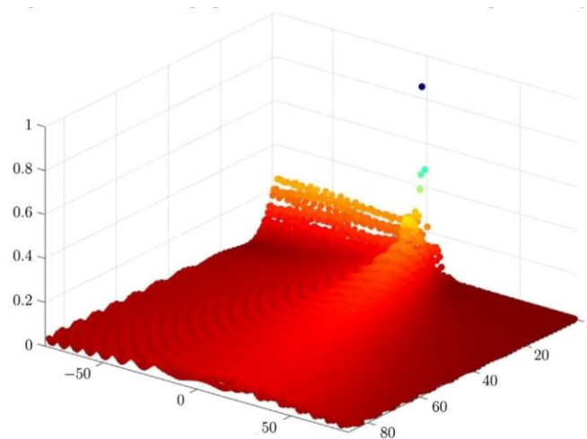
Non-symmetric propagation of Rayleigh waves.
